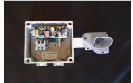
Sealed NEMA 4 Enclosure with Cable/Coax Strain Reliefs
